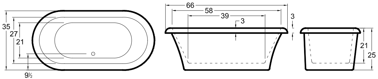
All bathtub dimensions are ± 1/2".
