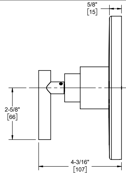
(TO-PB2L-66 SHOWN)
