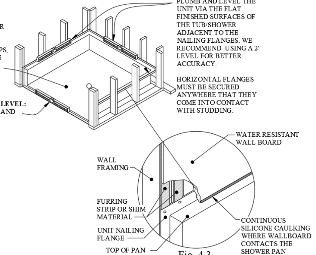
Fig. 4.3 Detail at Top of Pan (Installed under wallboard)
