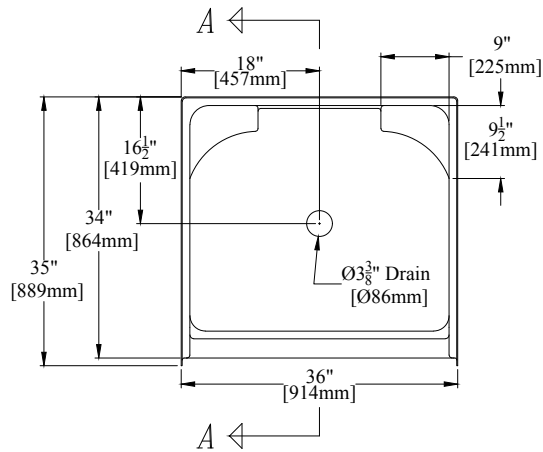
36" [914mm] 3-Piece Shower w/ 7" [178mm] Threshold & Molded Soap Ledges CENTER DRAIN
