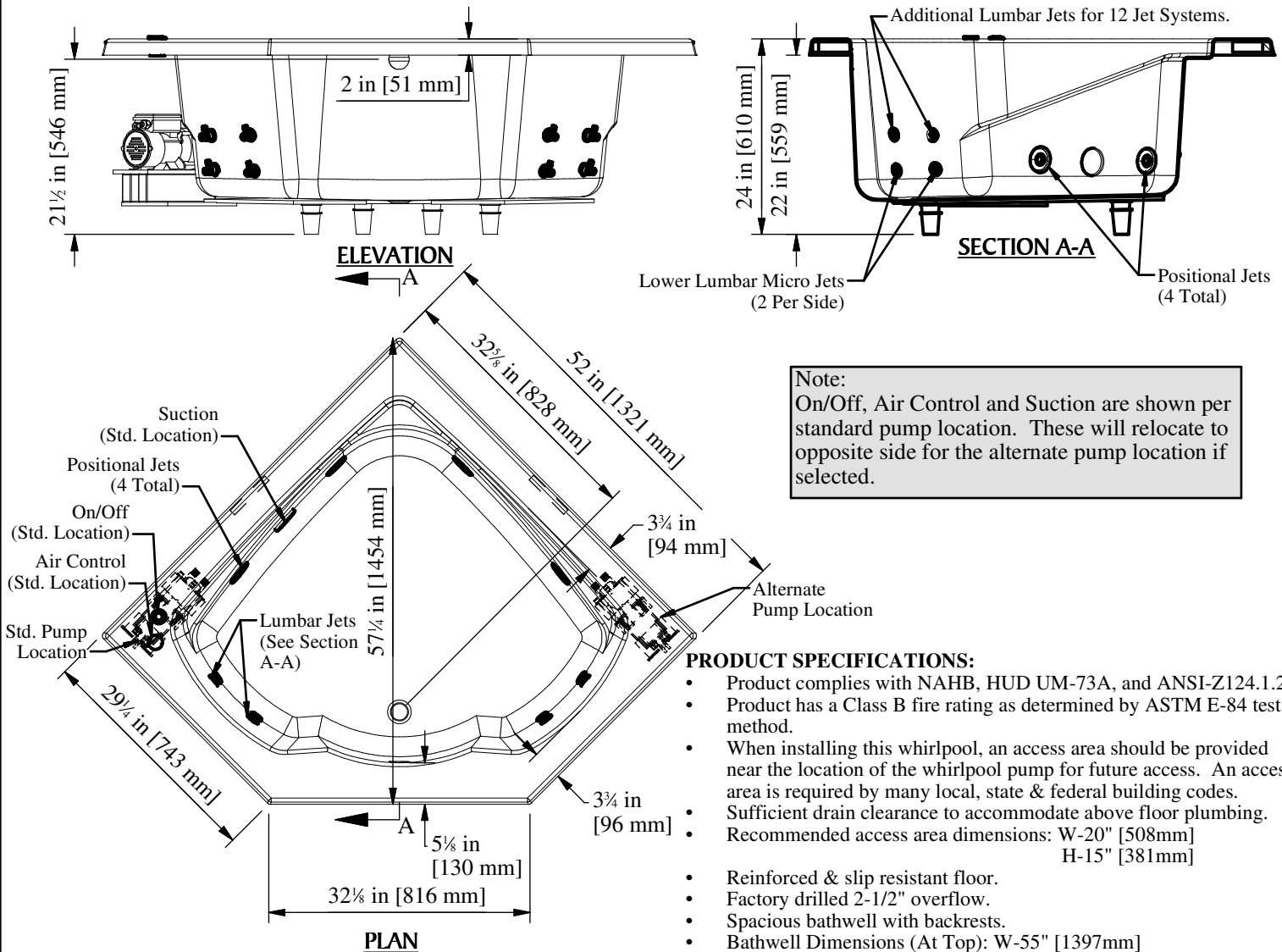
52" [1321 mm] Drop-In Bathtub w/ Molded Arm Rests & 8 or 12 Jet Whirlpool Package
