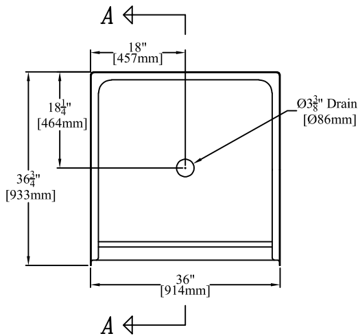
36" [914mm] Barrier-Free Shower w/ 2" [51mm] Threshold
